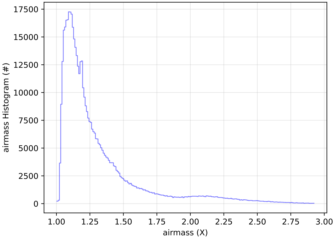
ddf_acor_sf10_lsf20_lsr10_v3.4_10yrs WFD i band: airmass Histogram
