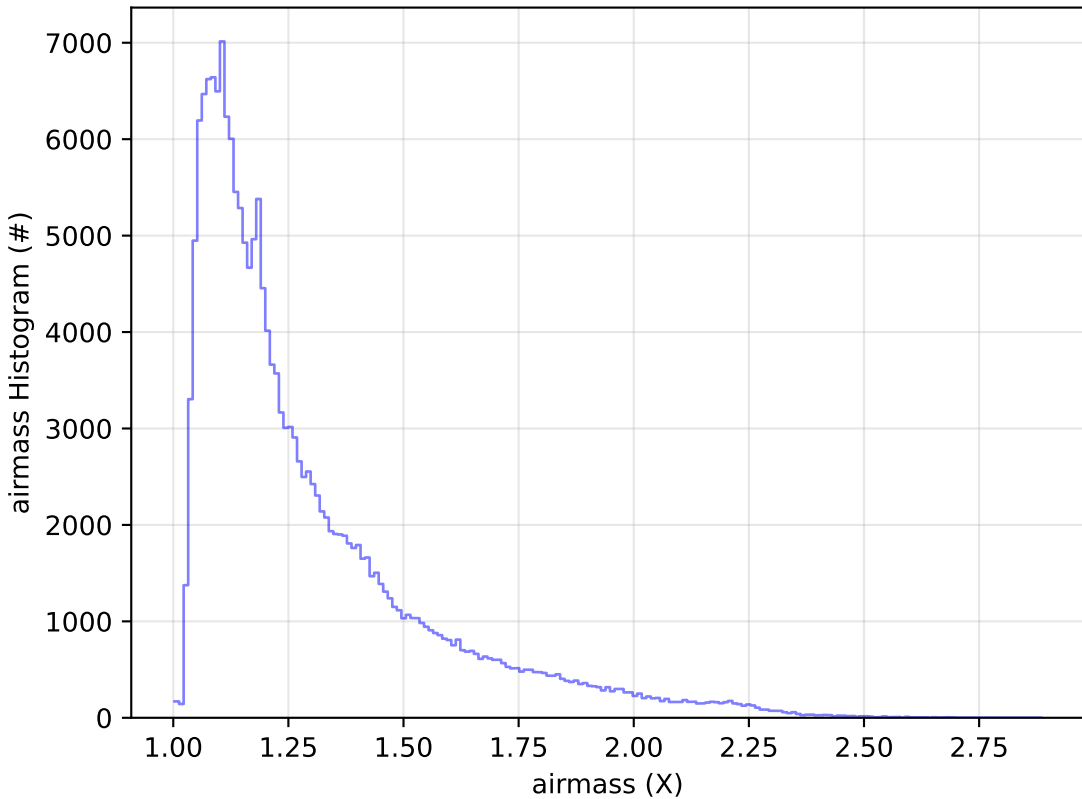
ddf_acor_sf10_lsf20_lsr10_v3.4_10yrs WFD g band: airmass Histogram
