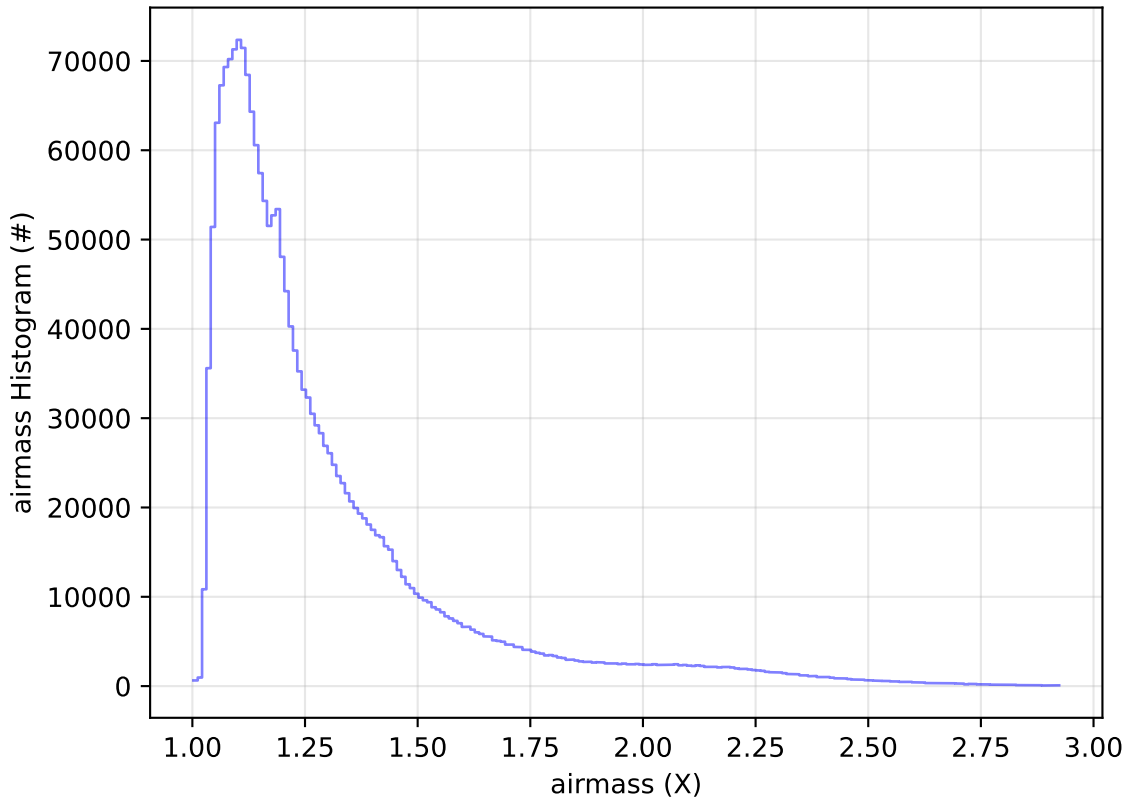
ddf_acor_sf10_lsf20_lsr10_v3.4_10yrs WFD all bands: airmass Histogram
