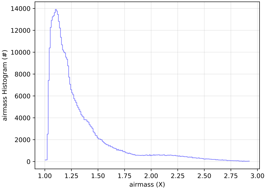
ddf_acor_sf10_lsf20_lsr10_v3.4_10yrs All sky z band: airmass Histogram
