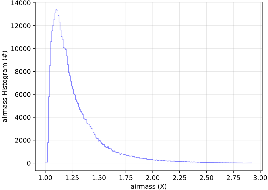
ddf_acor_sf10_lsf20_lsr10_v3.4_10yrs All sky y band: airmass Histogram
