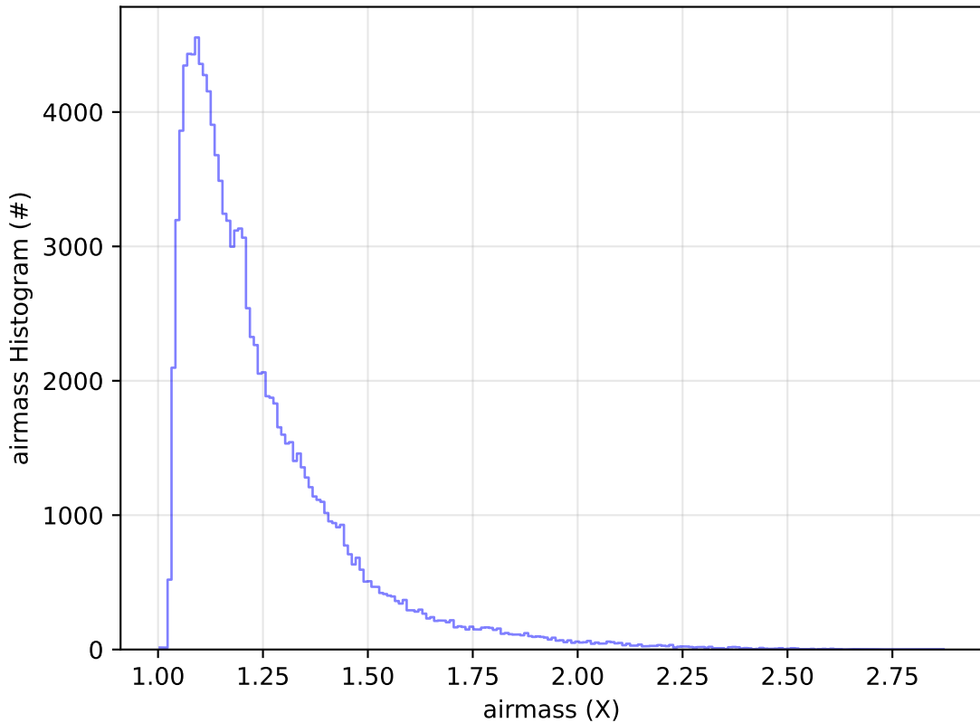
ddf_acor_sf10_lsf20_lsr10_v3.4_10yrs All sky u band: airmass Histogram
