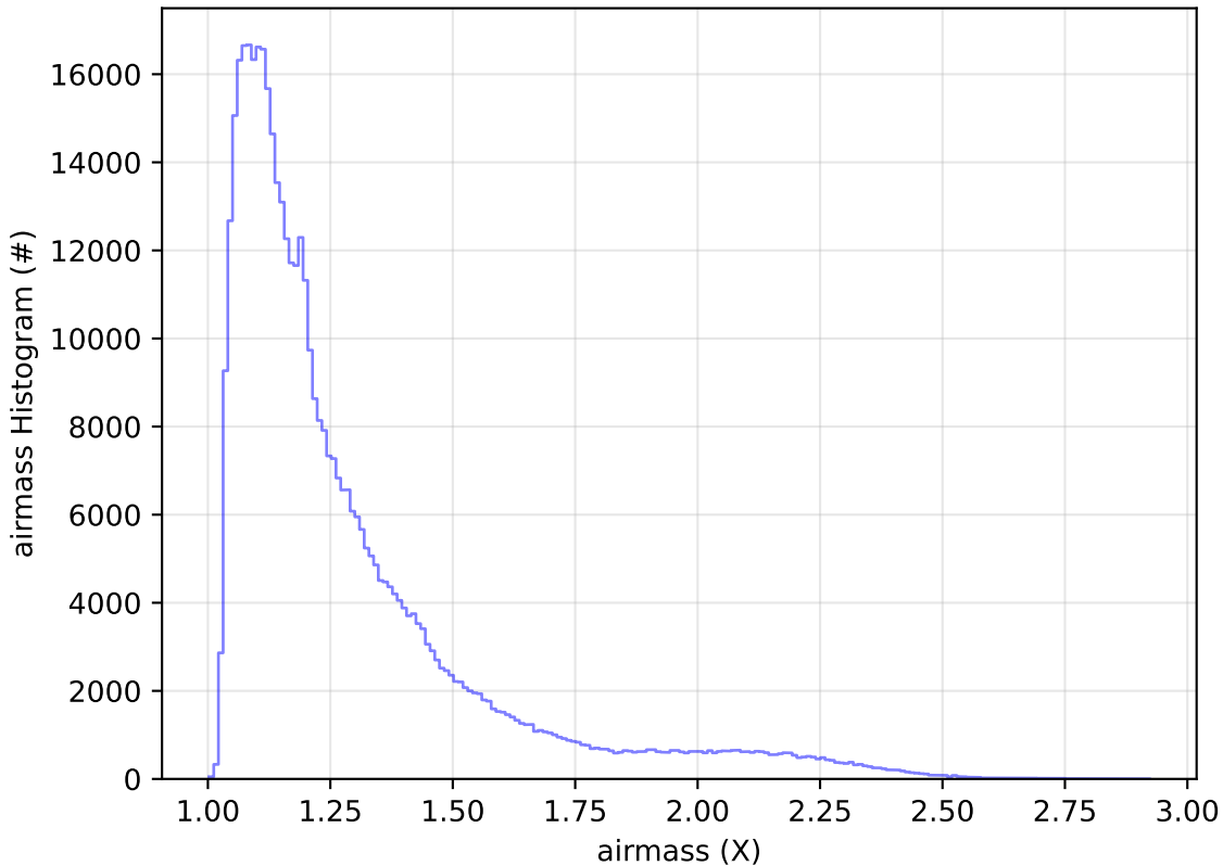
ddf_acor_sf10_lsf20_lsr10_v3.4_10yrs All sky r band: airmass Histogram
