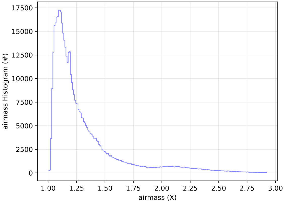
ddf_acor_sf10_lsf20_lsr10_v3.4_10yrs All sky i band: airmass Histogram
