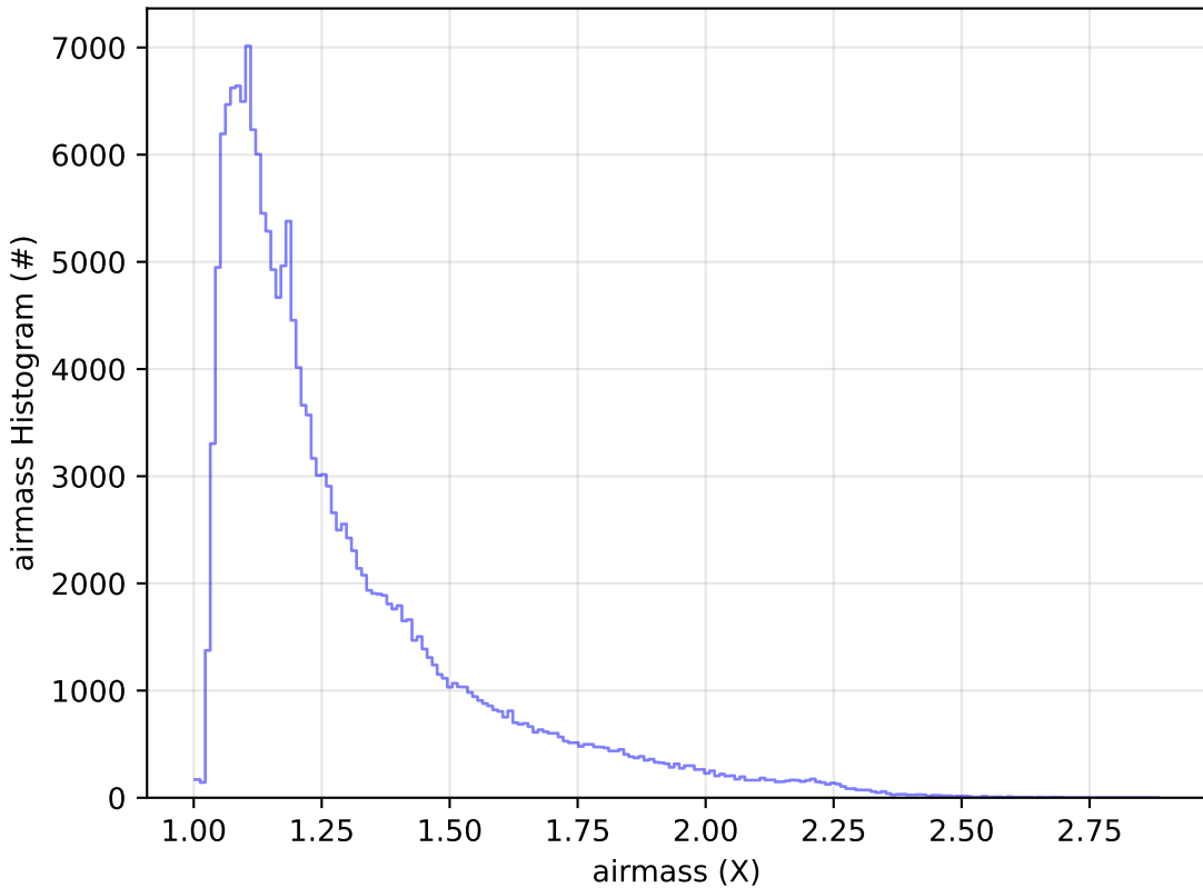
ddf_acor_sf10_lsf20_lsr10_v3.4_10yrs All sky g band: airmass Histogram
