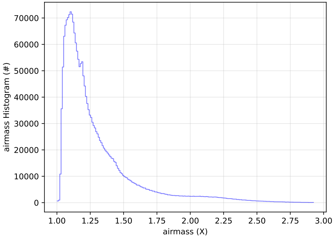
ddf_acor_sf10_lsf20_lsr10_v3.4_10yrs All sky all bands: airmass Histogram
