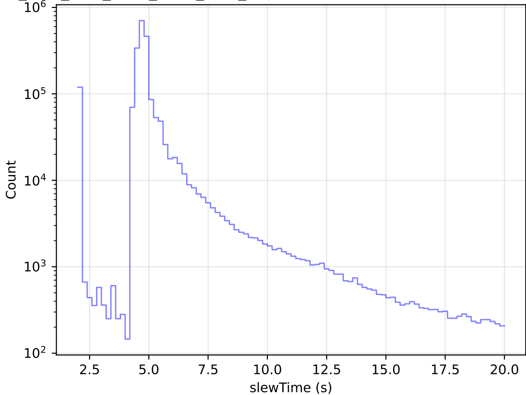
ddf_acor_sf10_lsf20_lsr10_v3.4_10yrs All visits: Zoom Slew Time Histogram
