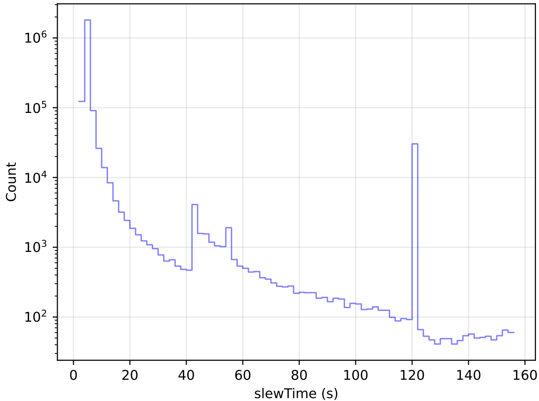
ddf_acor_sf10_lsf20_lsr10_v3.4_10yrs All visits: Slew Time Histogram
