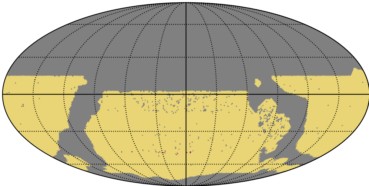
ddf_acor_sf10_lsf20_lsr10_v3.4_10yrs WFD: RapidRevisits
