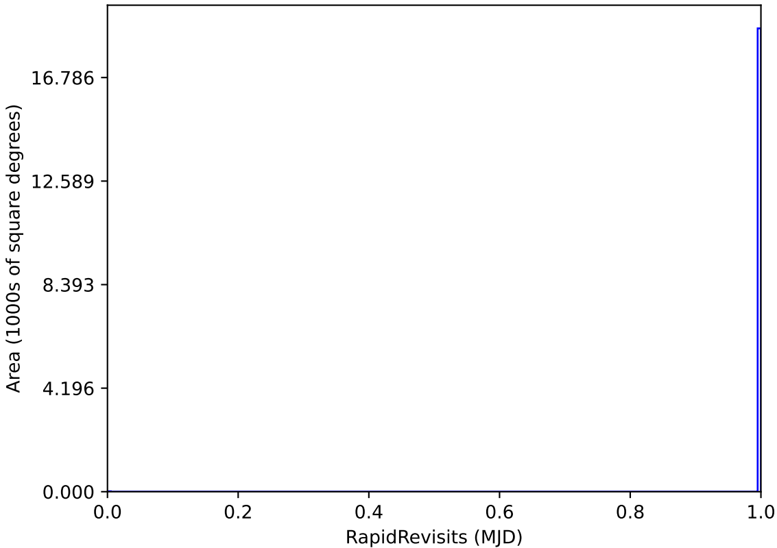
ddf_acor_sf10_lsf20_lsr10_v3.4_10yrs WFD: RapidRevisits
