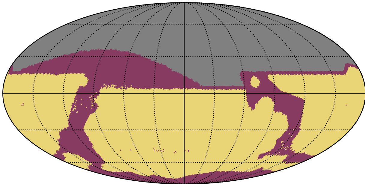
ddf_acor_sf10_lsf20_lsr10_v3.4_10yrs All sky: RapidRevisits
