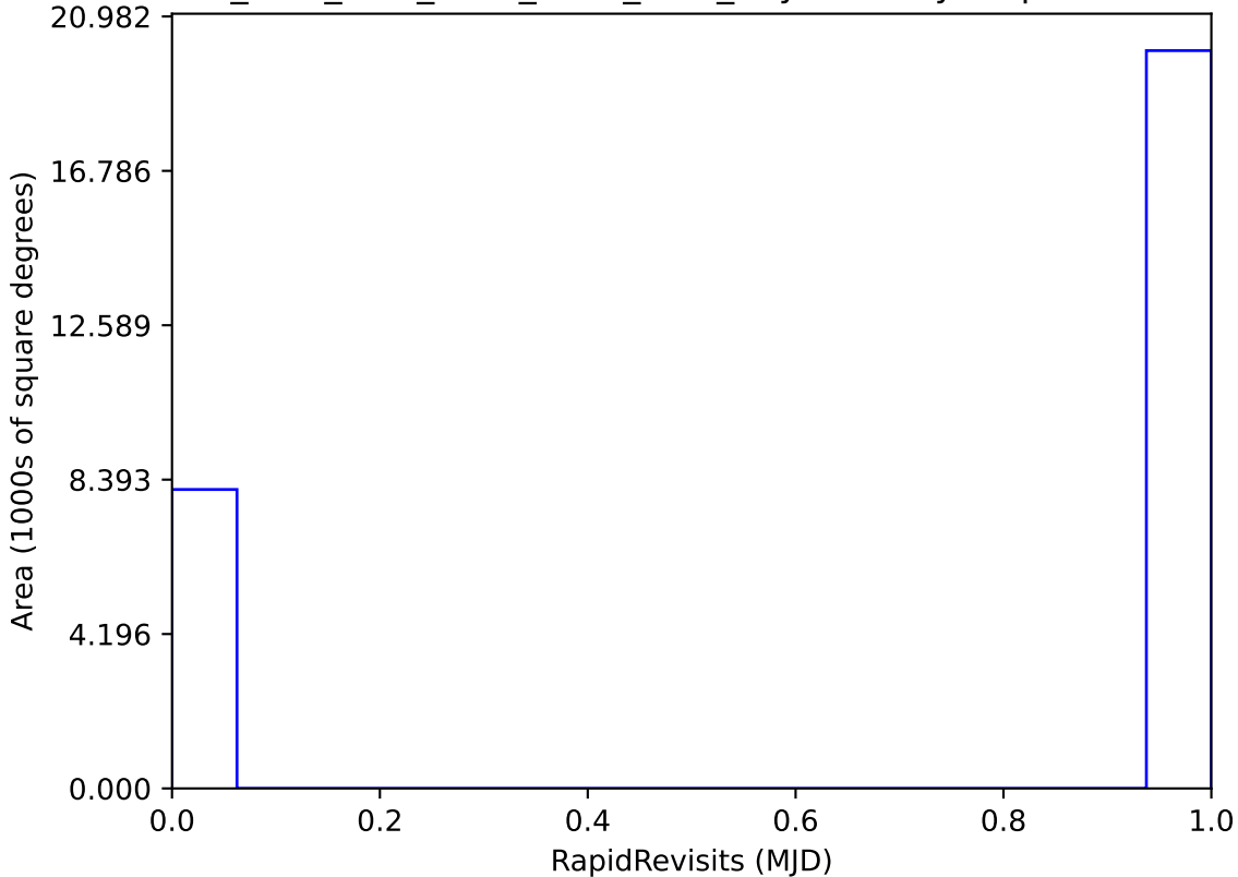
ddf_acor_sf10_lsf20_lsr10_v3.4_10yrs All sky: RapidRevisits
