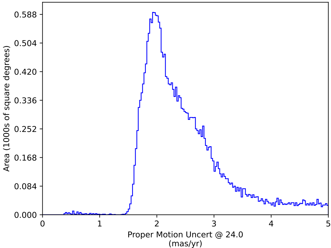
ddf_acor_sf10_lsf20_lsr10_v3.4_10yrs All sky: Proper Motion Uncert @ 24.0
