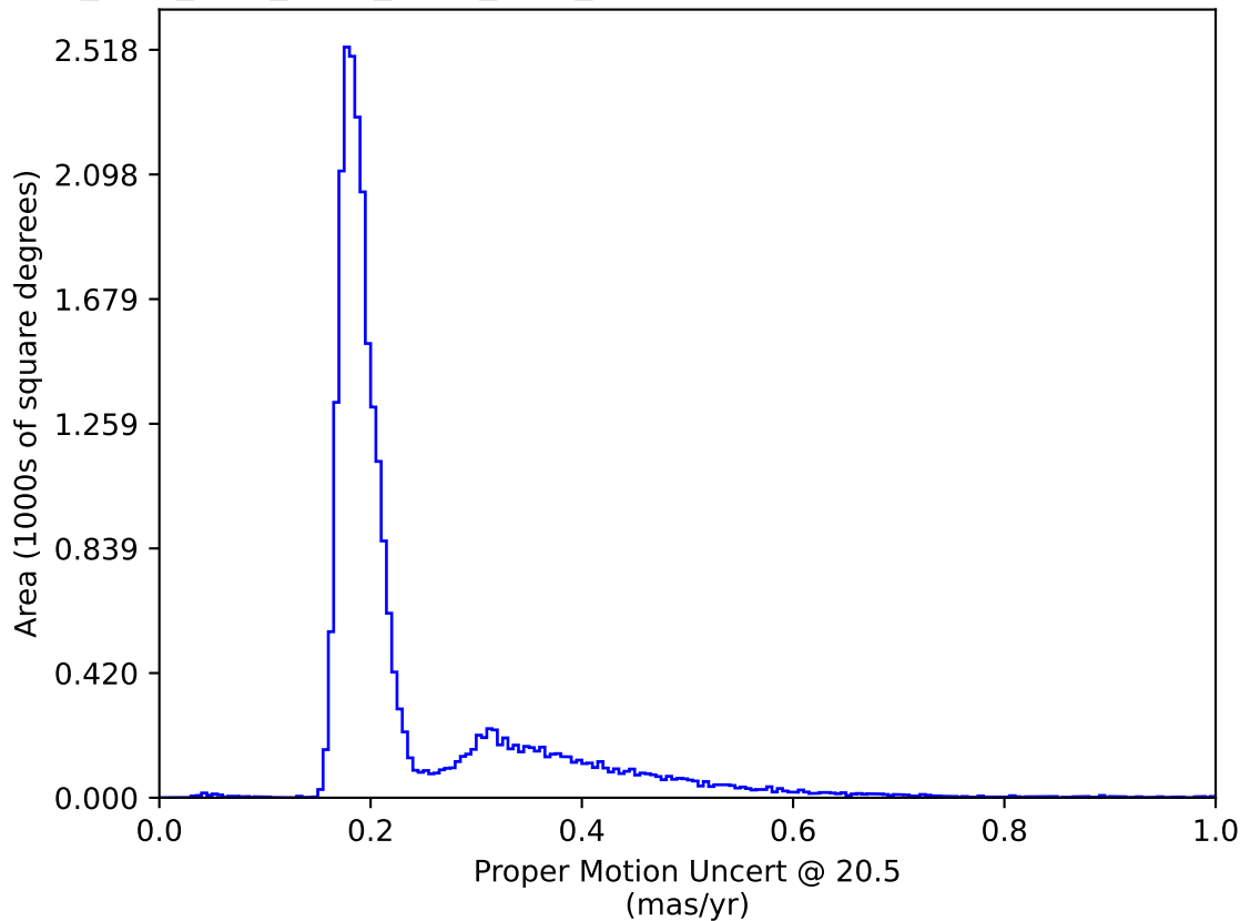
ddf_acor_sf10_lsf20_lsr10_v3.4_10yrs All sky: Proper Motion Uncert @ 20.5
