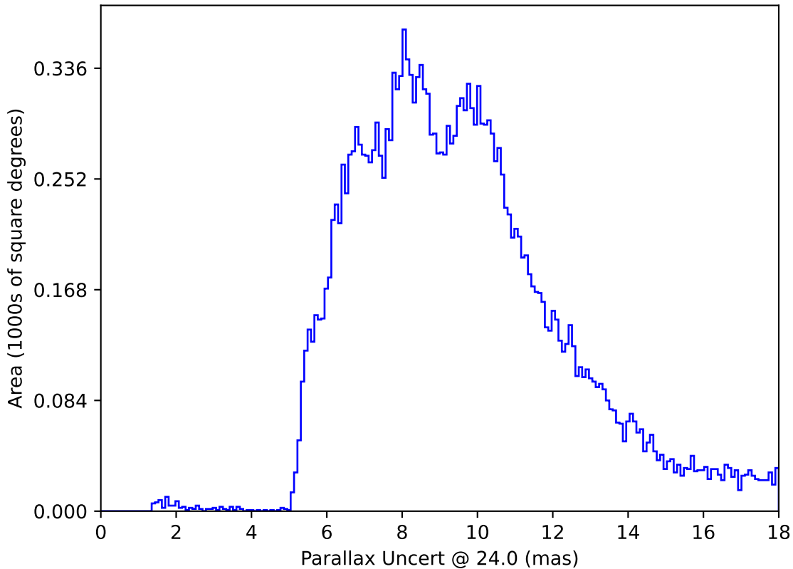
ddf_acor_sf10_lsf20_lsr10_v3.4_10yrs All sky: Parallax Uncert @ 24.0
