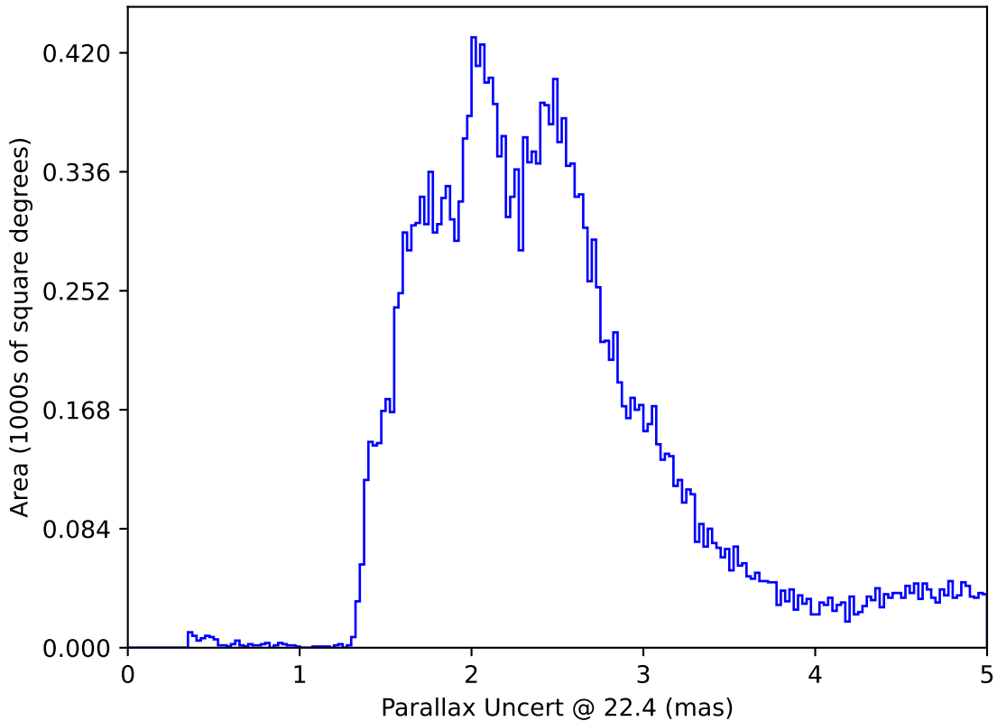
ddf_acor_sf10_lsf20_lsr10_v3.4_10yrs All sky: Parallax Uncert @ 22.4
