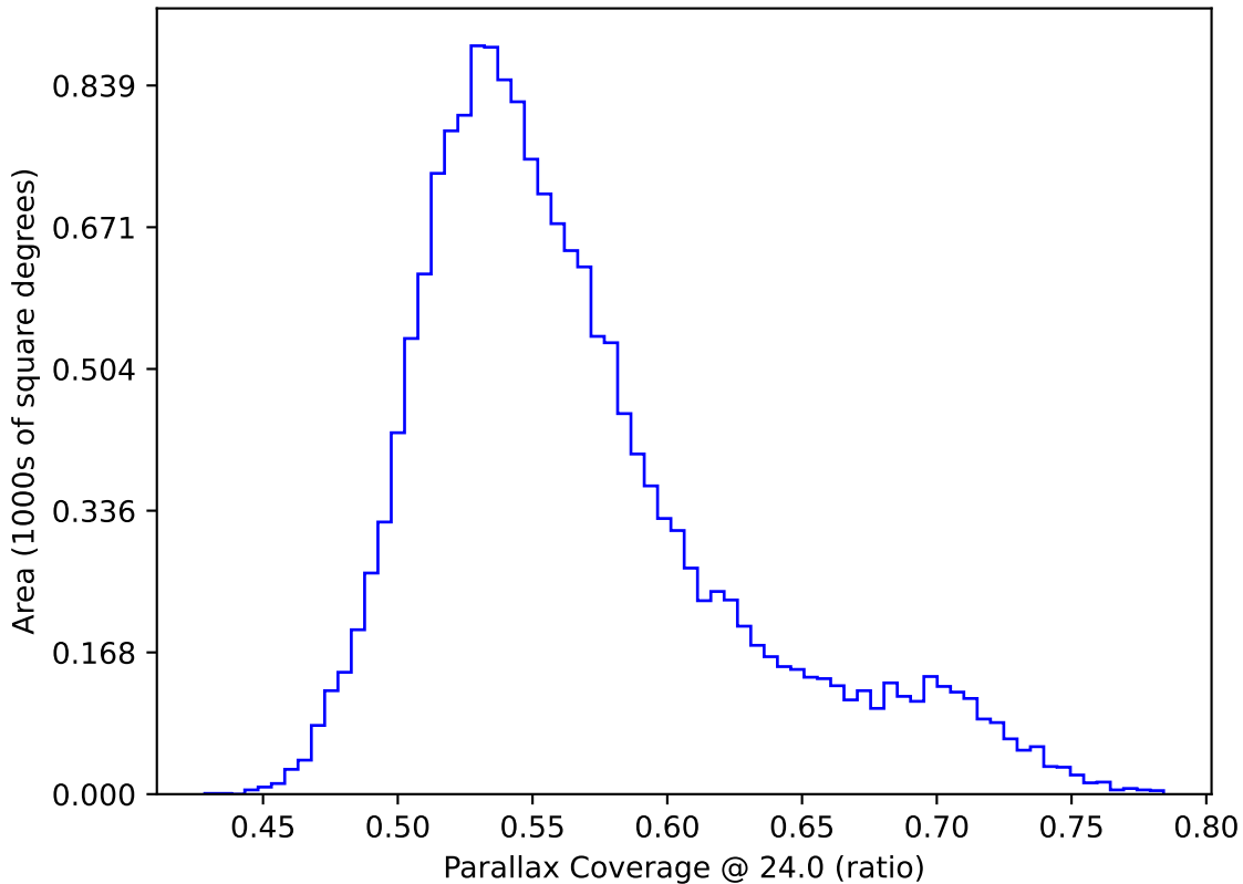
ddf_acor_sf10_lsf20_lsr10_v3.4_10yrs WFD: Parallax Coverage @ 24.0
