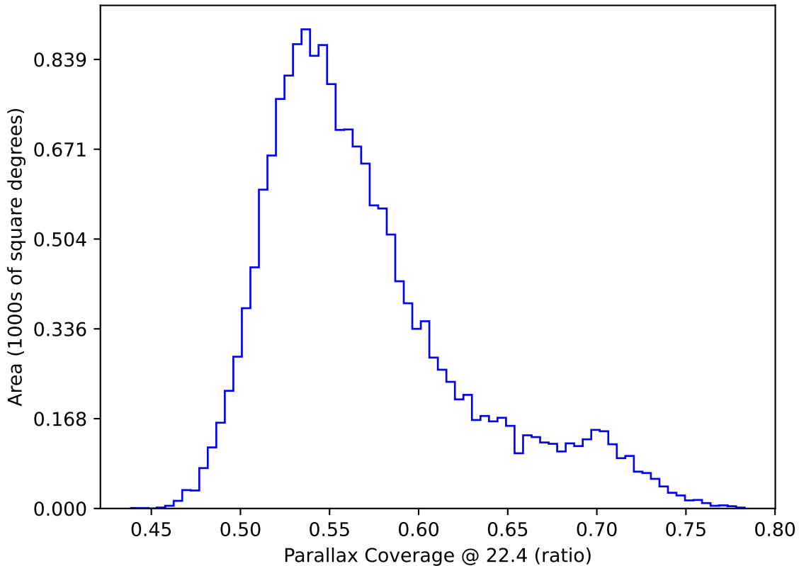
ddf_acor_sf10_lsf20_lsr10_v3.4_10yrs WFD: Parallax Coverage @ 22.4
