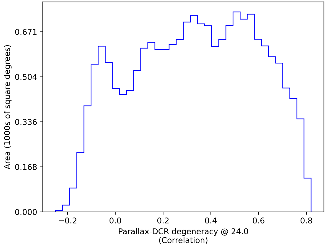
ddf_acor_sf10_lsf20_lsr10_v3.4_10yrs WFD: Parallax-DCR degeneracy @ 24.0
