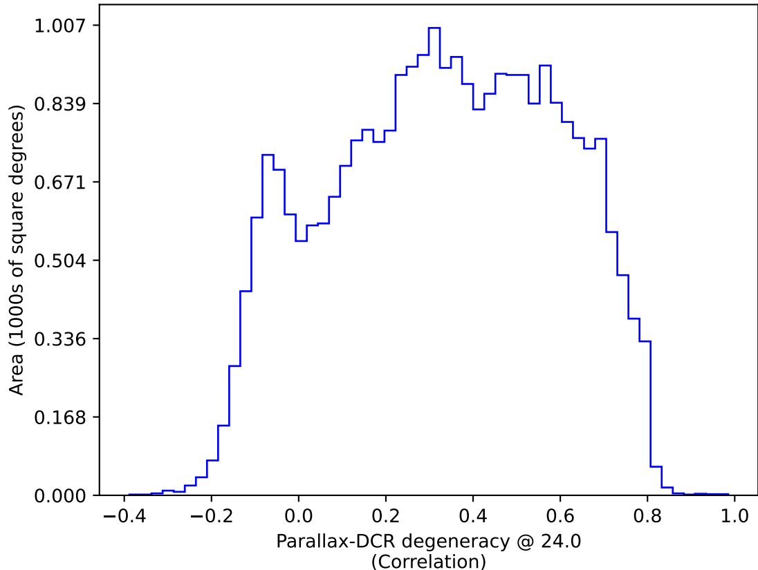
ddf_acor_sf10_lsf20_lsr10_v3.4_10yrs All sky: Parallax-DCR degeneracy @ 24.0
