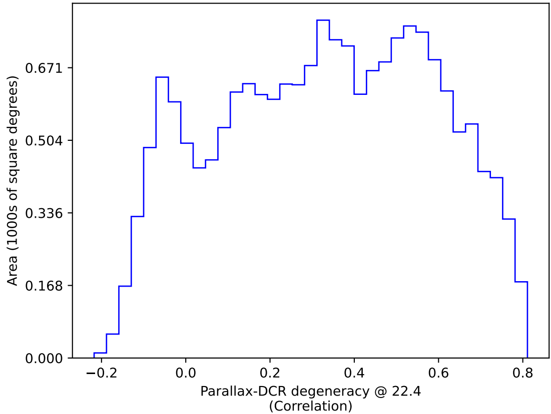
ddf_acor_sf10_lsf20_lsr10_v3.4_10yrs WFD: Parallax-DCR degeneracy @ 22.4
