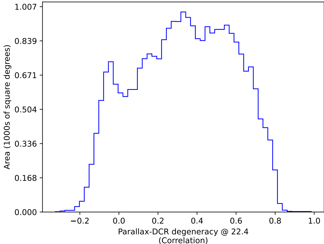
ddf_acor_sf10_lsf20_lsr10_v3.4_10yrs All sky: Parallax-DCR degeneracy @ 22.4
