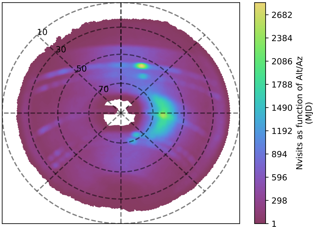
ddf_acor_sf10_lsf20_lsr10_v3.4_10yrs z band: Nvisits as function of Alt/Az
