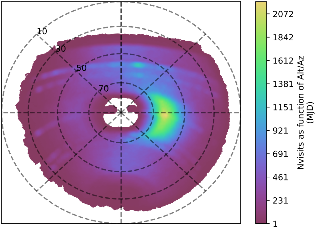
ddf_acor_sf10_lsf20_lsr10_v3.4_10yrs y band: Nvisits as function of Alt/Az
