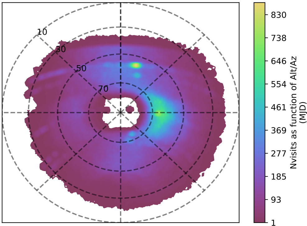
ddf_acor_sf10_lsf20_lsr10_v3.4_10yrs u band: Nvisits as function of Alt/Az
