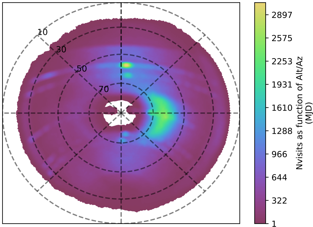
ddf_acor_sf10_lsf20_lsr10_v3.4_10yrs i band: Nvisits as function of Alt/Az
