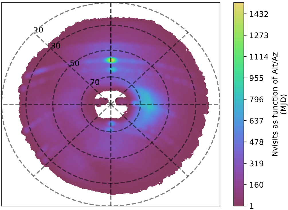
ddf_acor_sf10_lsf20_lsr10_v3.4_10yrs g band: Nvisits as function of Alt/Az
