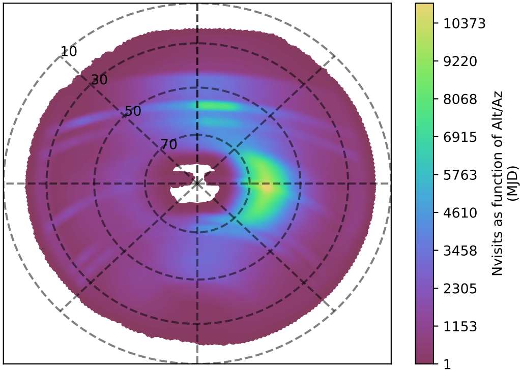
ddf_acor_sf10_lsf20_lsr10_v3.4_10yrs all bands: Nvisits as function of Alt/Az
