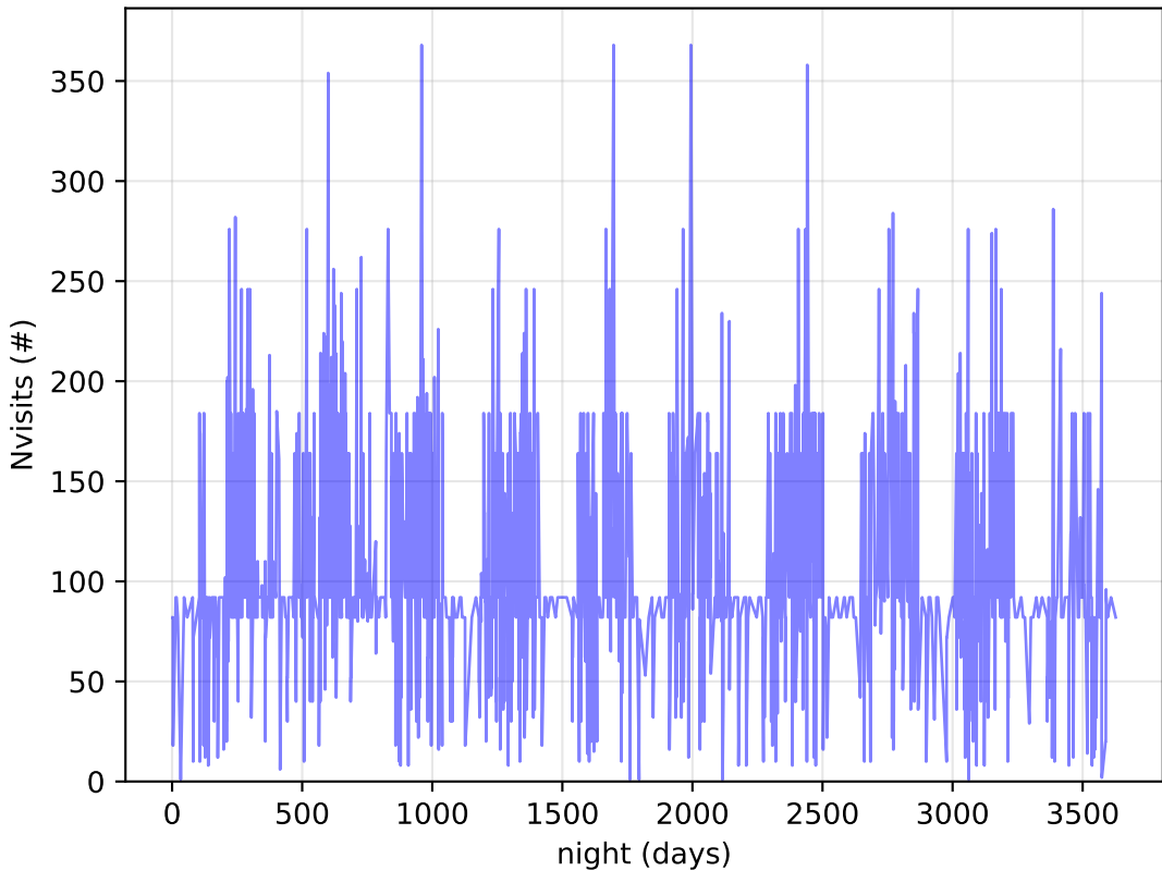
ddf_acor_sf10_ls10_lsr10_v3.4_10yrs DDF: Nvisits
