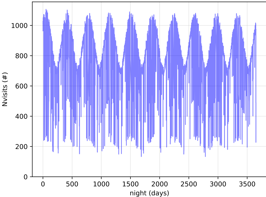
ddf_acor_sf10_ls10_lsr10_v3.4_10yrs All visits: Nvisits
