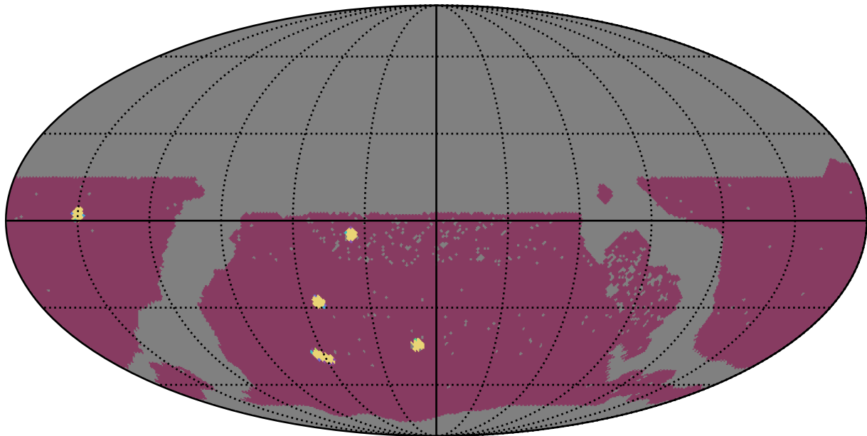
ddf_acor_sf10_lsf20_lsr10_v3.4_10yrs WFD: NumberOfQuickRevisits
