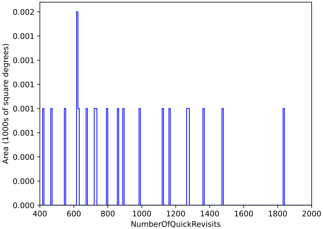
ddf_acor_sf10_lsf20_lsr10_v3.4_10yrs WFD: NumberOfQuickRevisits
