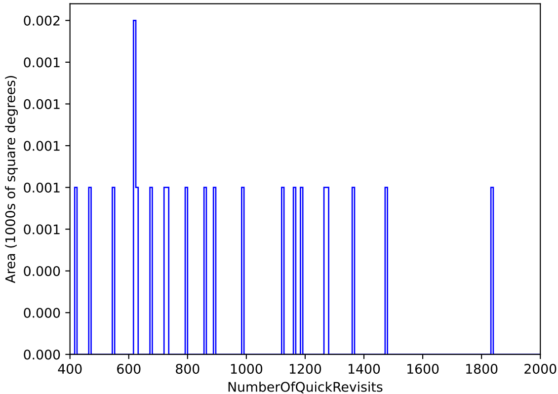
ddf_acor_sf10_lsf20_lsr10_v3.4_10yrs All sky: NumberOfQuickRevisits
