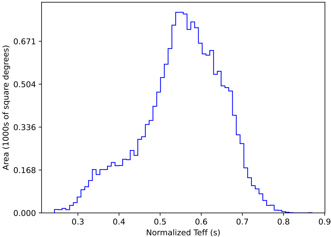
ddf_acor_sf10_lsf20_lsr10_v3.4_10yrs WFD y band: Normalized Teff
