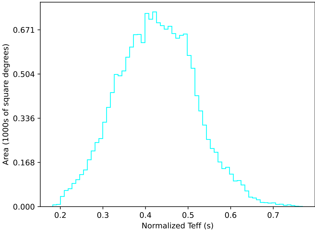
ddf_acor_sf10_lsf20_lsr10_v3.4_10yrs WFD u band: Normalized Teff
