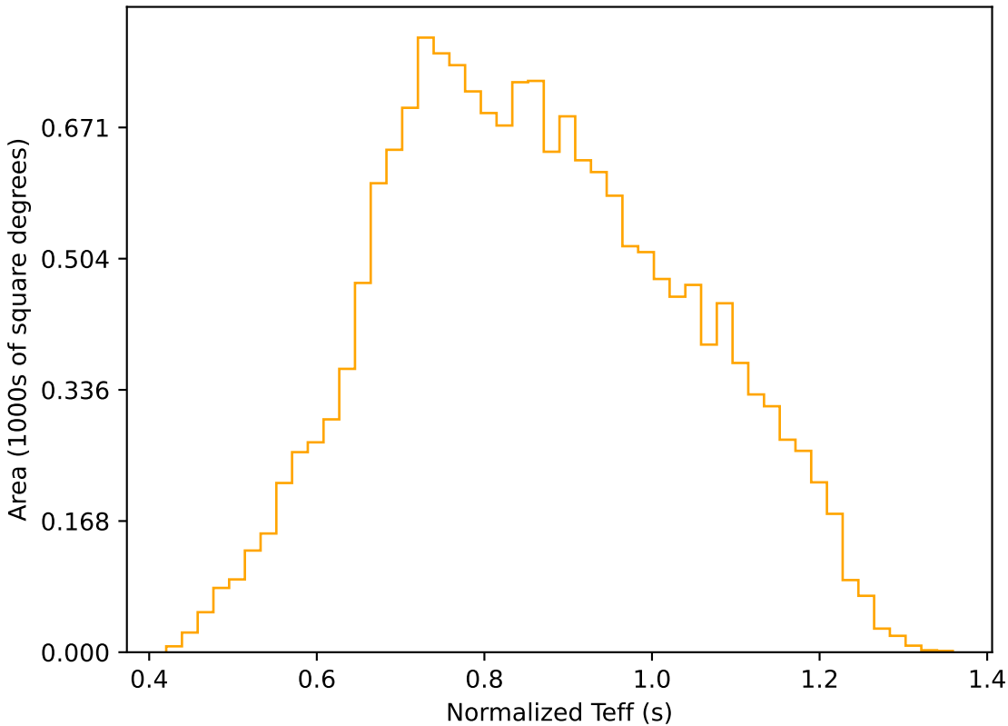
ddf_acor_sf10_lsf20_lsr10_v3.4_10yrs WFD r band: Normalized Teff
