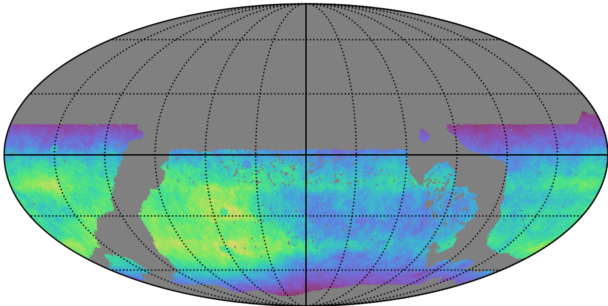
ddf_acor_sf10_lsf20_lsr10_v3.4_10yrs WFD i band: Normalized Teff
