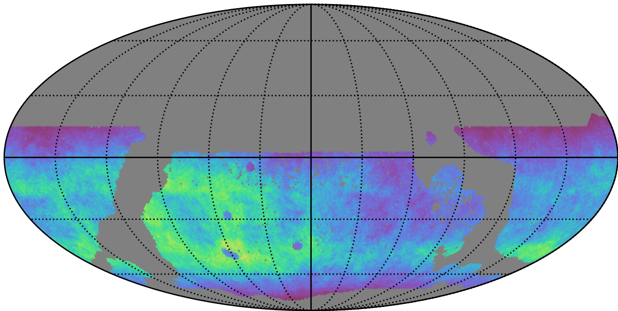
ddf_acor_sf10_lsf20_lsr10_v3.4_10yrs WFD g band: Normalized Teff
