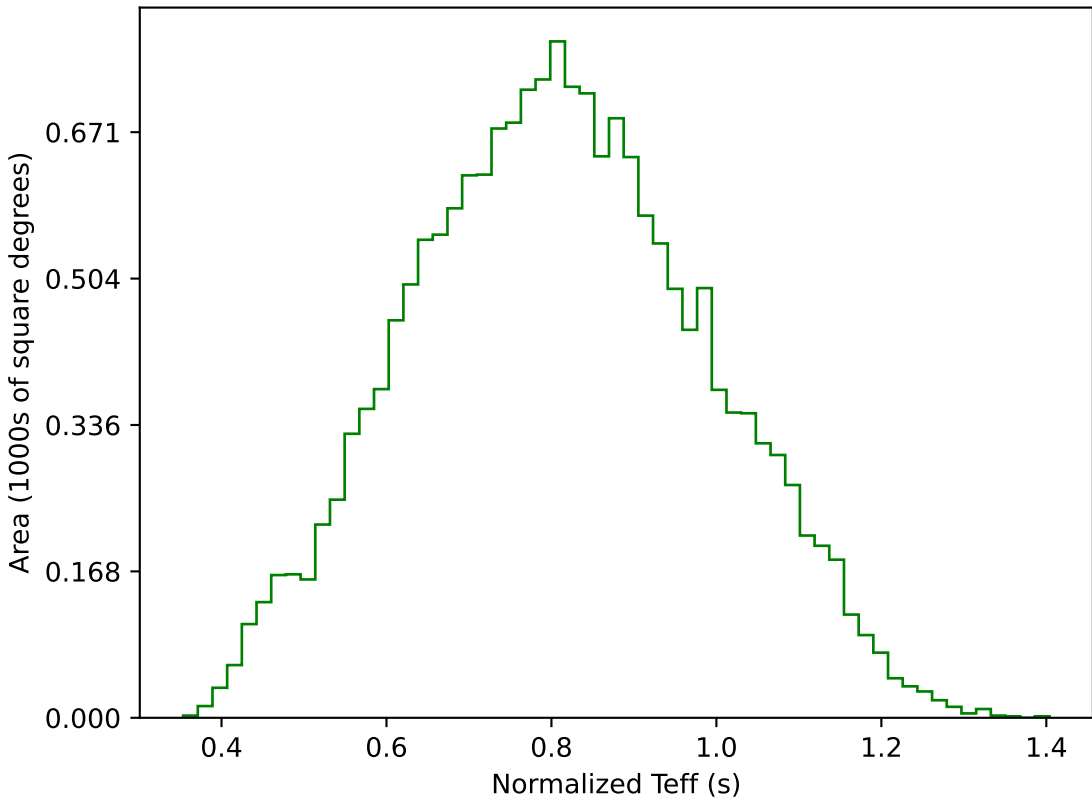
ddf_acor_sf10_lsf20_lsr10_v3.4_10yrs WFD g band: Normalized Teff
