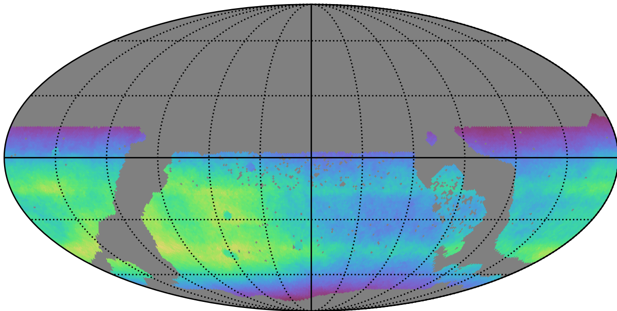
ddf_acor_sf10_lsf20_lsr10_v3.4_10yrs WFD all bands: Normalized Teff
