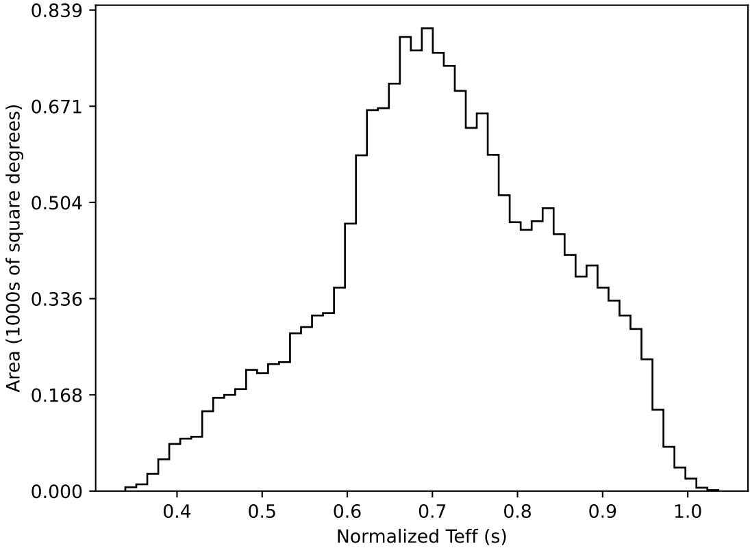
ddf_acor_sf10_lsf20_lsr10_v3.4_10yrs WFD all bands: Normalized Teff
