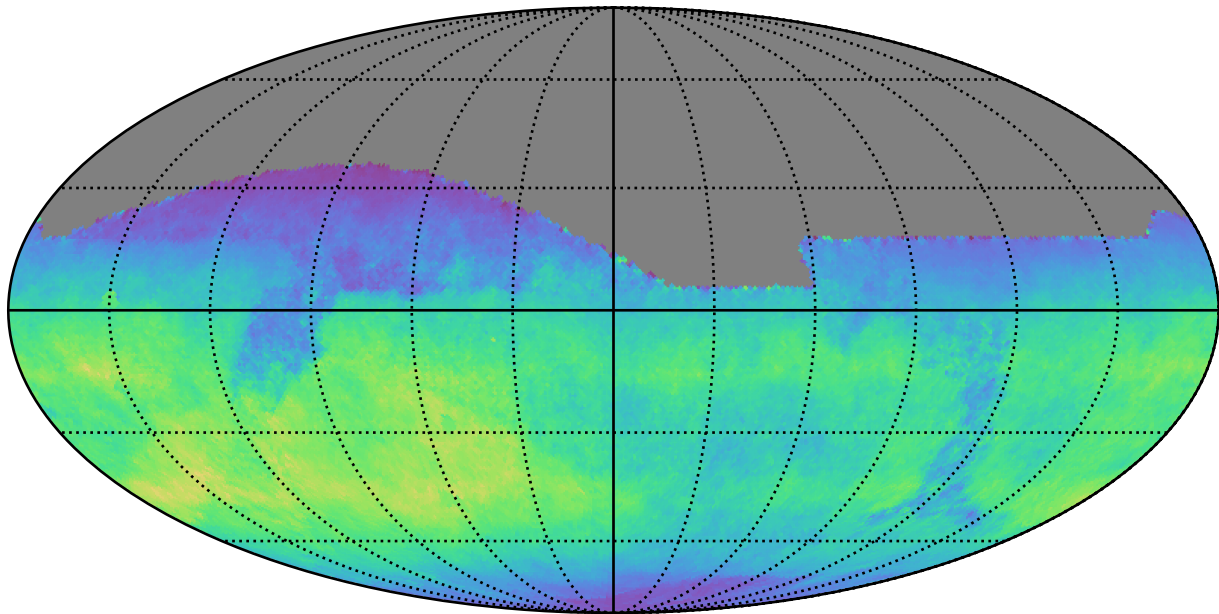
ddf_acor_sf10_lsf20_lsr10_v3.4_10yrs All sky z band: Normalized Teff
