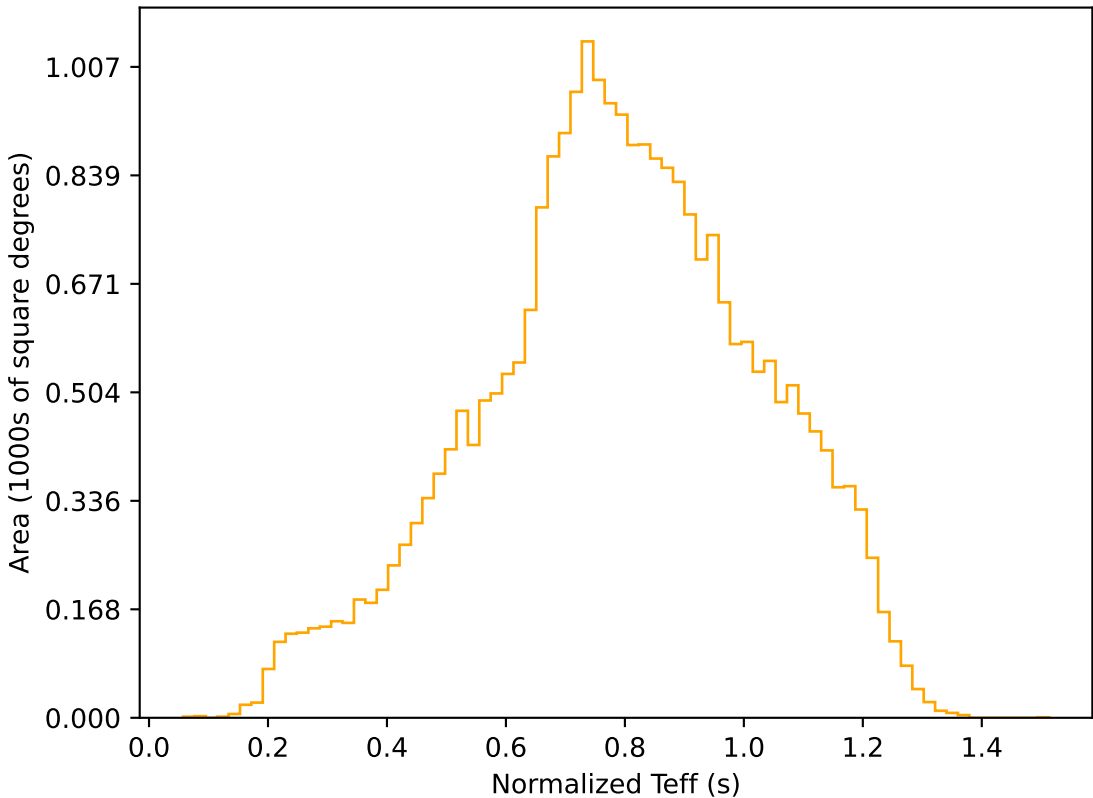
ddf_acor_sf10_lsf20_lsr10_v3.4_10yrs All sky r band: Normalized Teff
