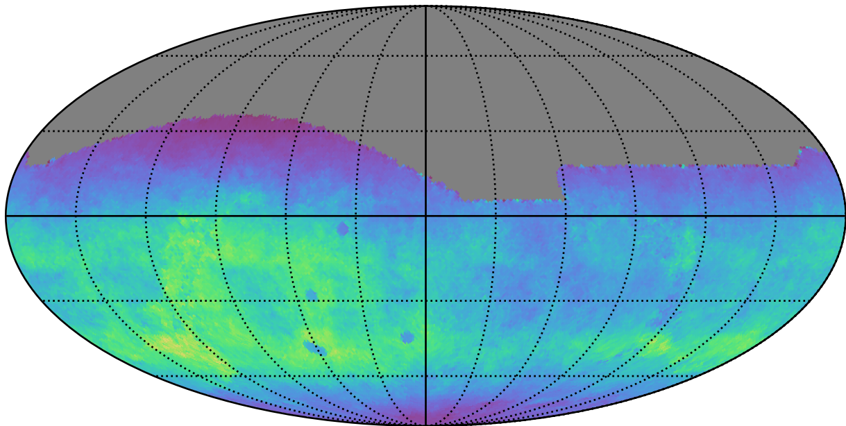
ddf_acor_sf10_lsf20_lsr10_v3.4_10yrs All sky g band: Normalized Teff
