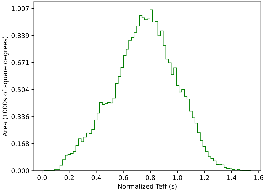
ddf_acor_sf10_lsf20_lsr10_v3.4_10yrs All sky g band: Normalized Teff
