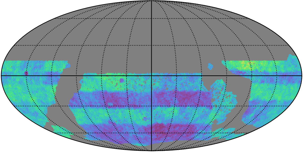
ddf_acor_sf10_lsf20_lsr10_v3.4_10yrs WFD: Normalized Proper Motion Uncert @ 24.0
